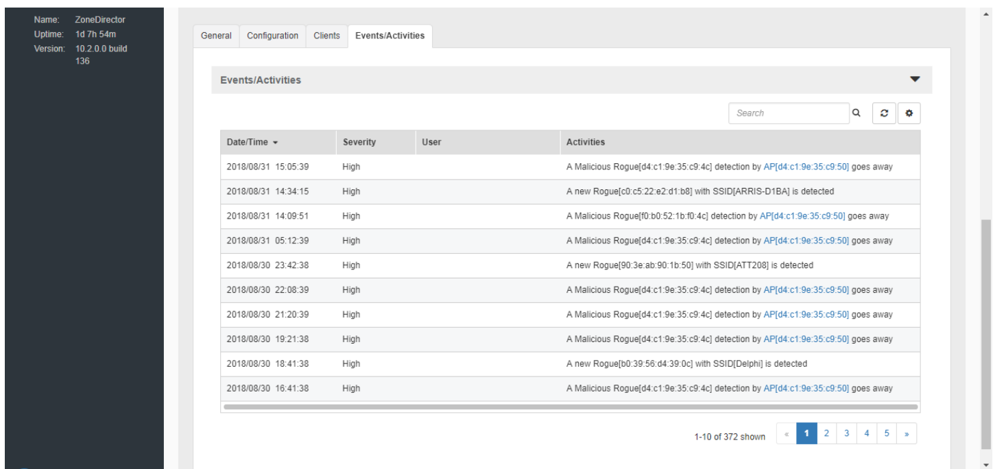
FIGURE 281 AP-specific events
